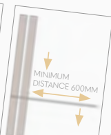
2. Soakaway should be at least 600mm from the wall to avoid causing damp to the footings.
